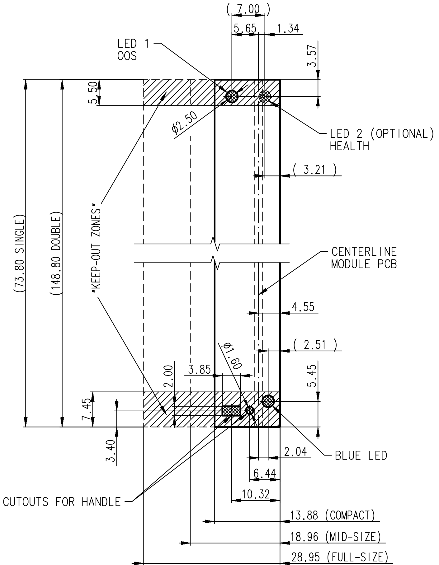
SCHROFF AMC MODULE FRONT PANEL w/ ROUND LEDs
