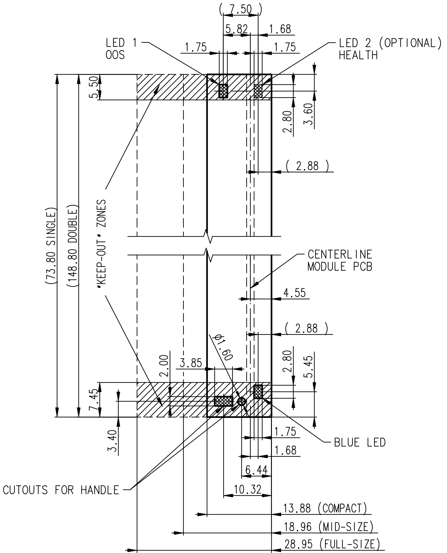
SCHROFF AMC MODULE FRONT PANEL w/ RECTANGULAR LEDs
