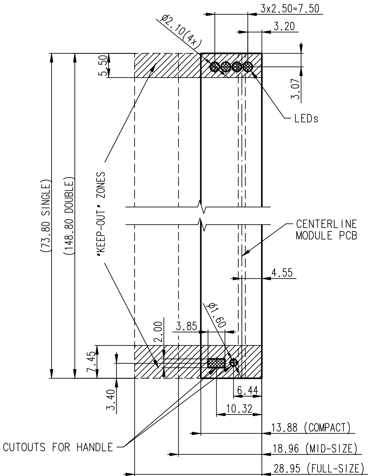
SCHROFF AMC MODULE FRONT PANEL w/ 4x ROUND LEDs
